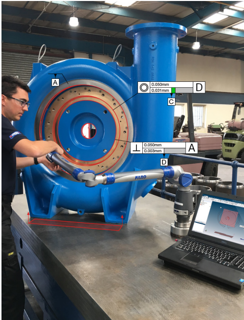
The ability to run FARO CAM2 from a portable laptop ensure maximum portability and flexibility.
